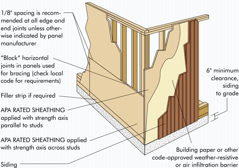
APA PANEL WALL SHEATHING
