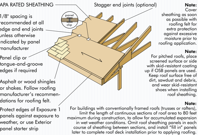
FIGURE 21 APA PANEL ROOF SHEATHING
