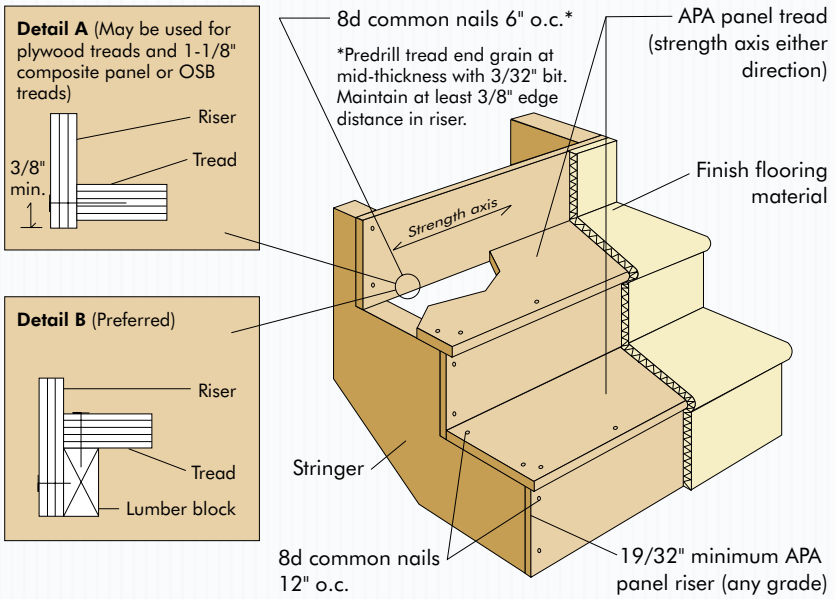
APA PANEL STAIR TREADS AND RISERS
