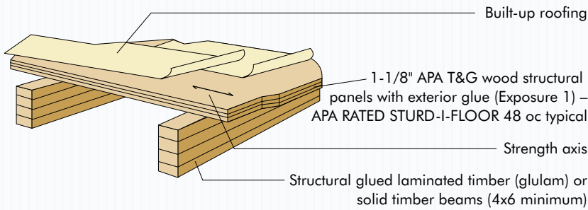
HEAVY TIMBER ROOF CONSTRUCTION
