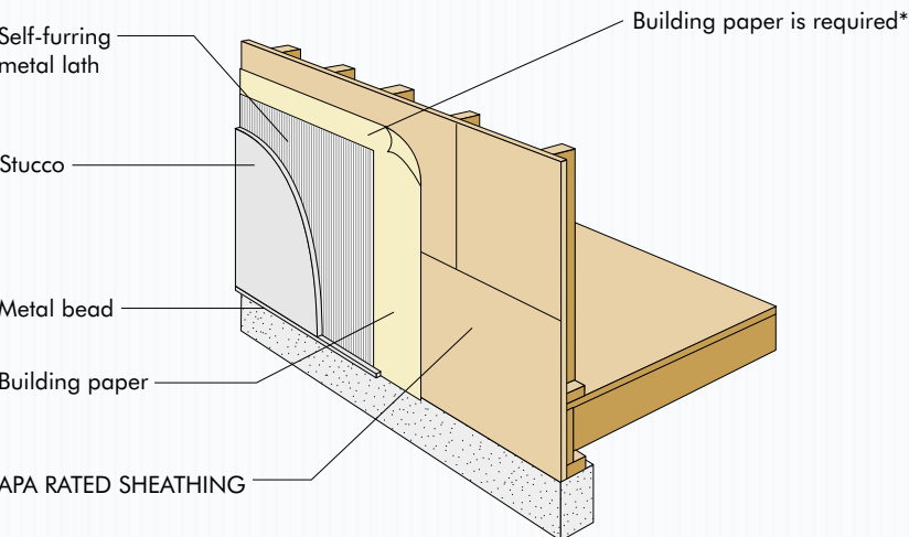
FIGURE 16 STUCCO OVER APA PANEL SHEATHING
